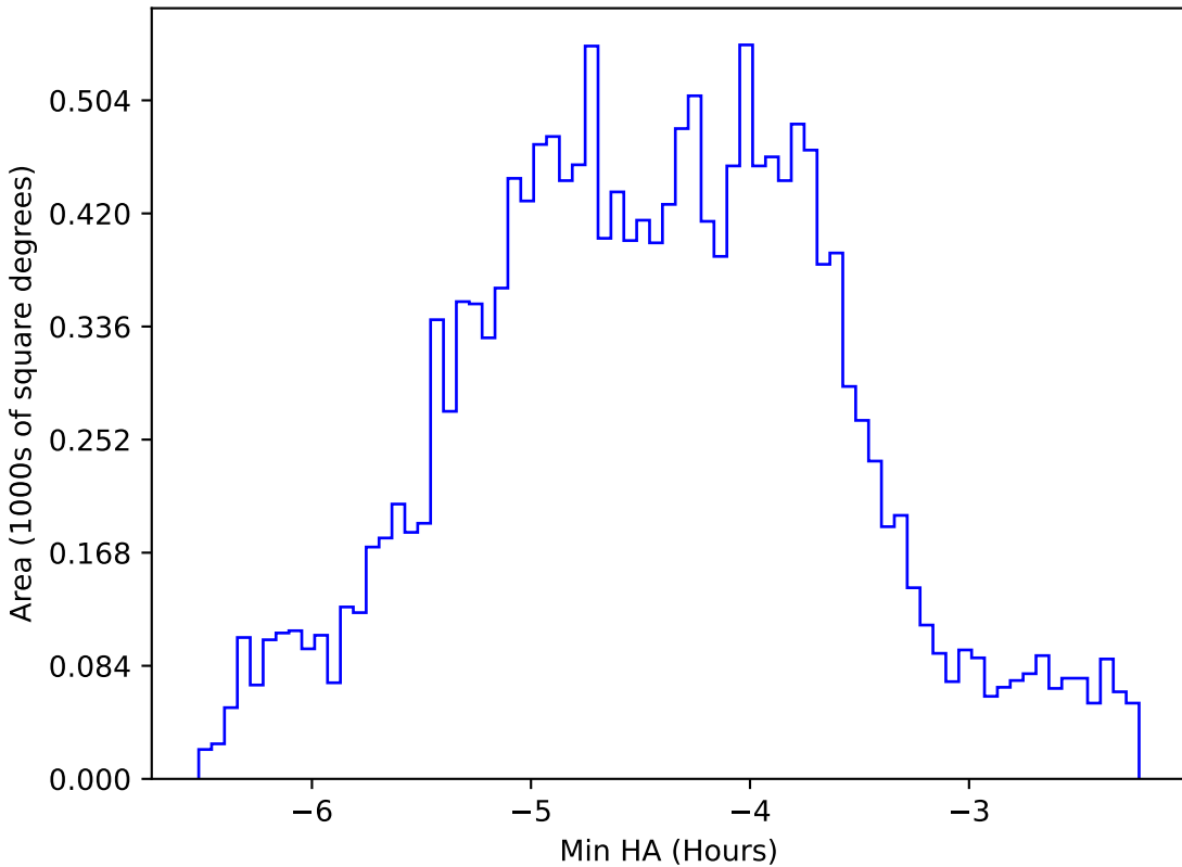
too_elab_r64_d2_gz_v3.4_10yrs WFD z band: Min HA
