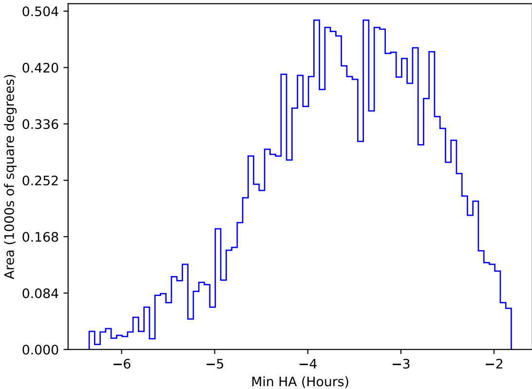
too_elab_r64_d2_gz_v3.4_10yrs WFD y band: Min HA
