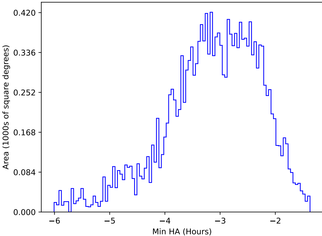
too_elab_r64_d2_gz_v3.4_10yrs WFD u band: Min HA
