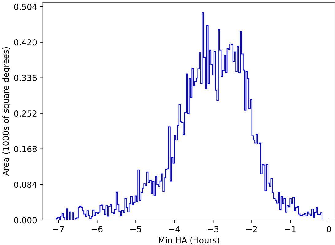
too_elab_r64_d2_gz_v3.4_10yrs All sky u band: Min HA
