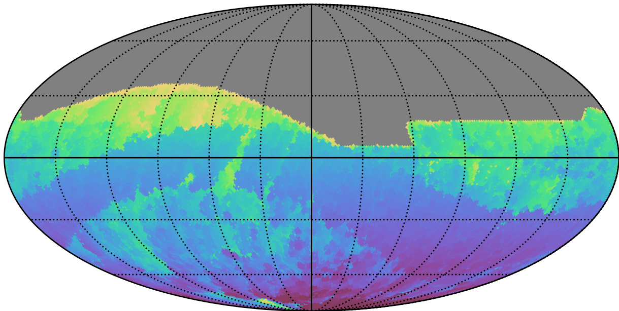
too_elab_r64_d2_gz_v3.4_10yrs All sky r band: Min HA
