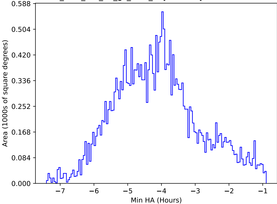
too_elab_r64_d2_gz_v3.4_10yrs All sky i band: Min HA
