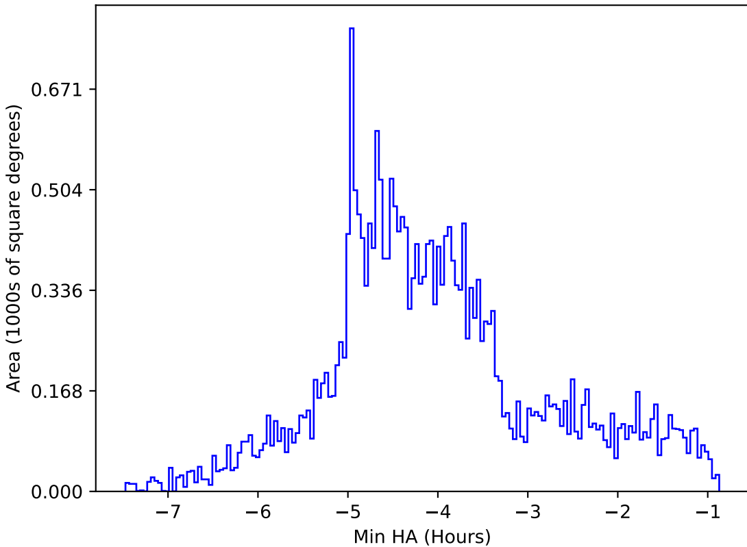
too_elab_r64_d2_gz_v3.4_10yrs All sky g band: Min HA
