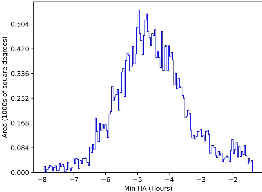
too_elab_r64_d2_gz_v3.4_10yrs All sky all bands: Min HA
