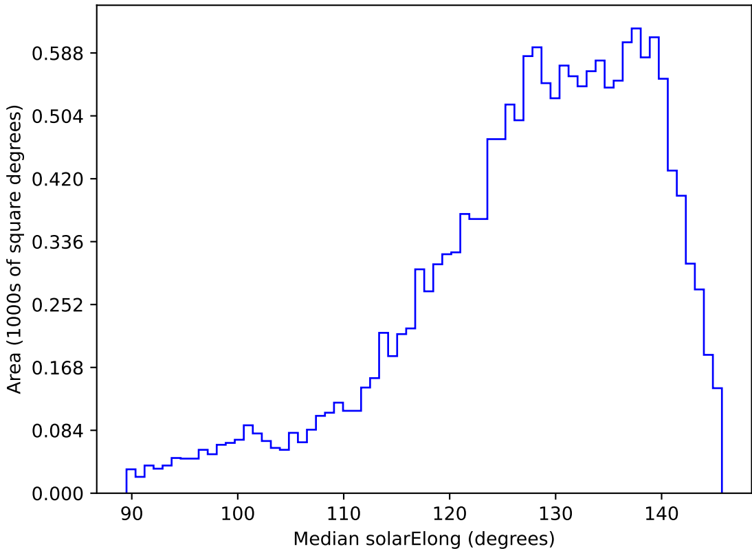
too_elab_r64_d2_gz_v3.4_10yrs WFD z band: Median solarElong
