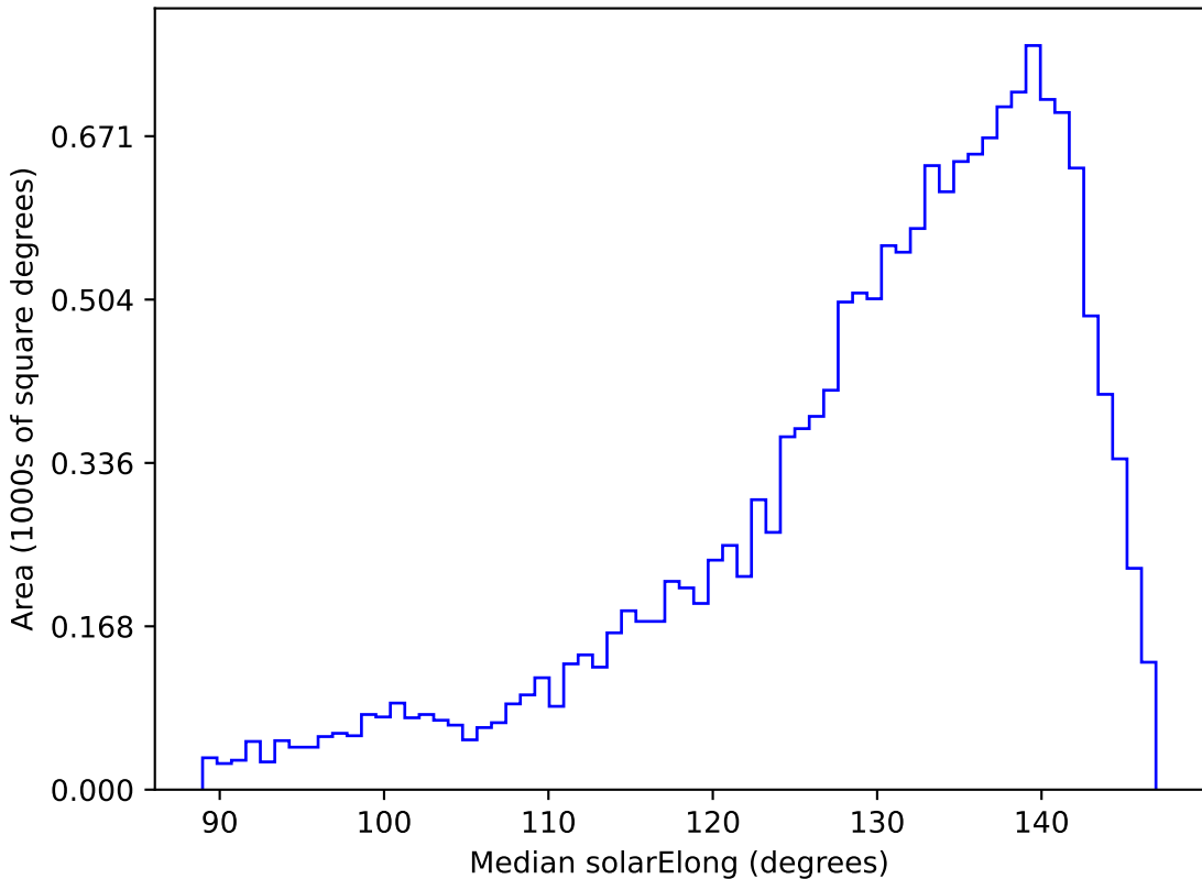
too_elab_r64_d2_gz_v3.4_10yrs WFD y band: Median solarElong
