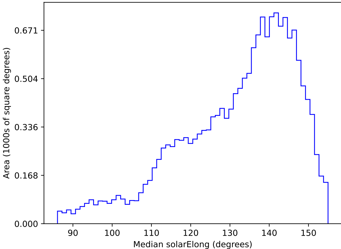
too_elab_r64_d2_gz_v3.4_10yrs WFD u band: Median solarElong
