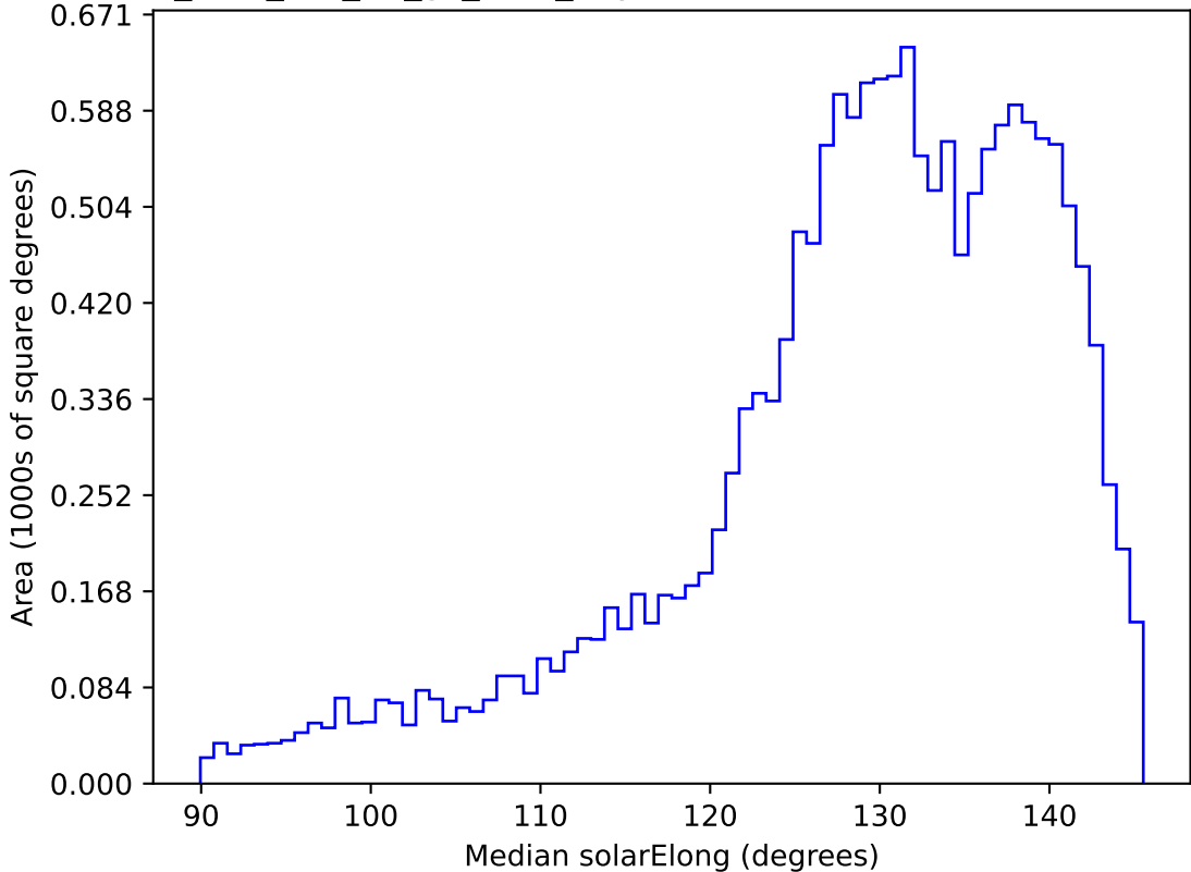
too_elab_r64_d2_gz_v3.4_10yrs WFD i band: Median solarElong
