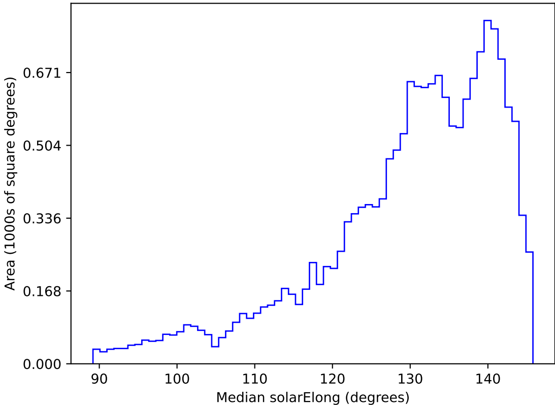
too_elab_r64_d2_gz_v3.4_10yrs WFD all bands: Median solarElong
