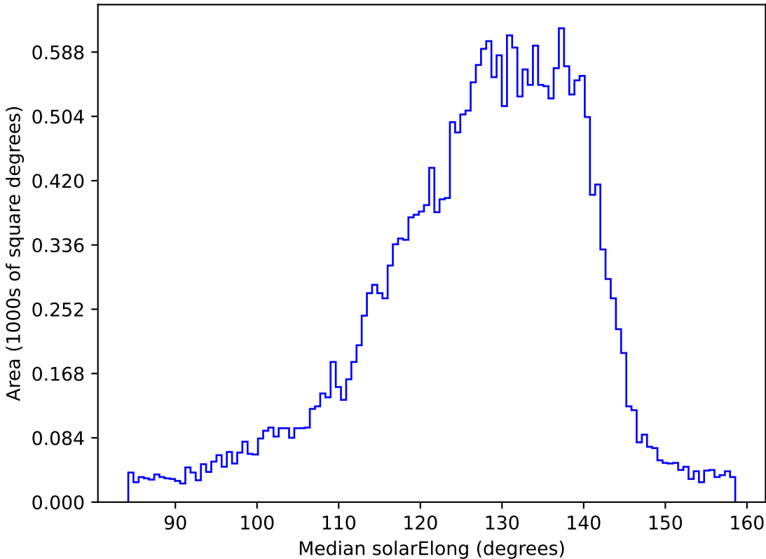
too_elab_r64_d2_gz_v3.4_10yrs All sky z band: Median solarElong
