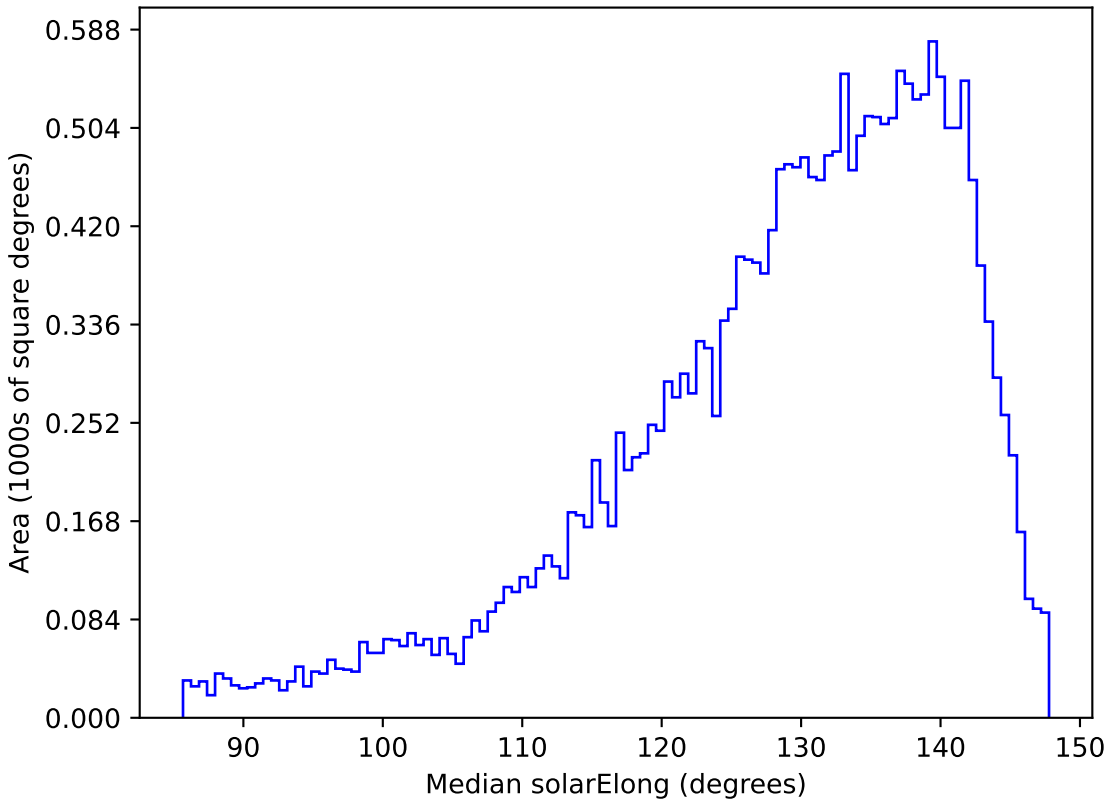
too_elab_r64_d2_gz_v3.4_10yrs All sky y band: Median solarElong
