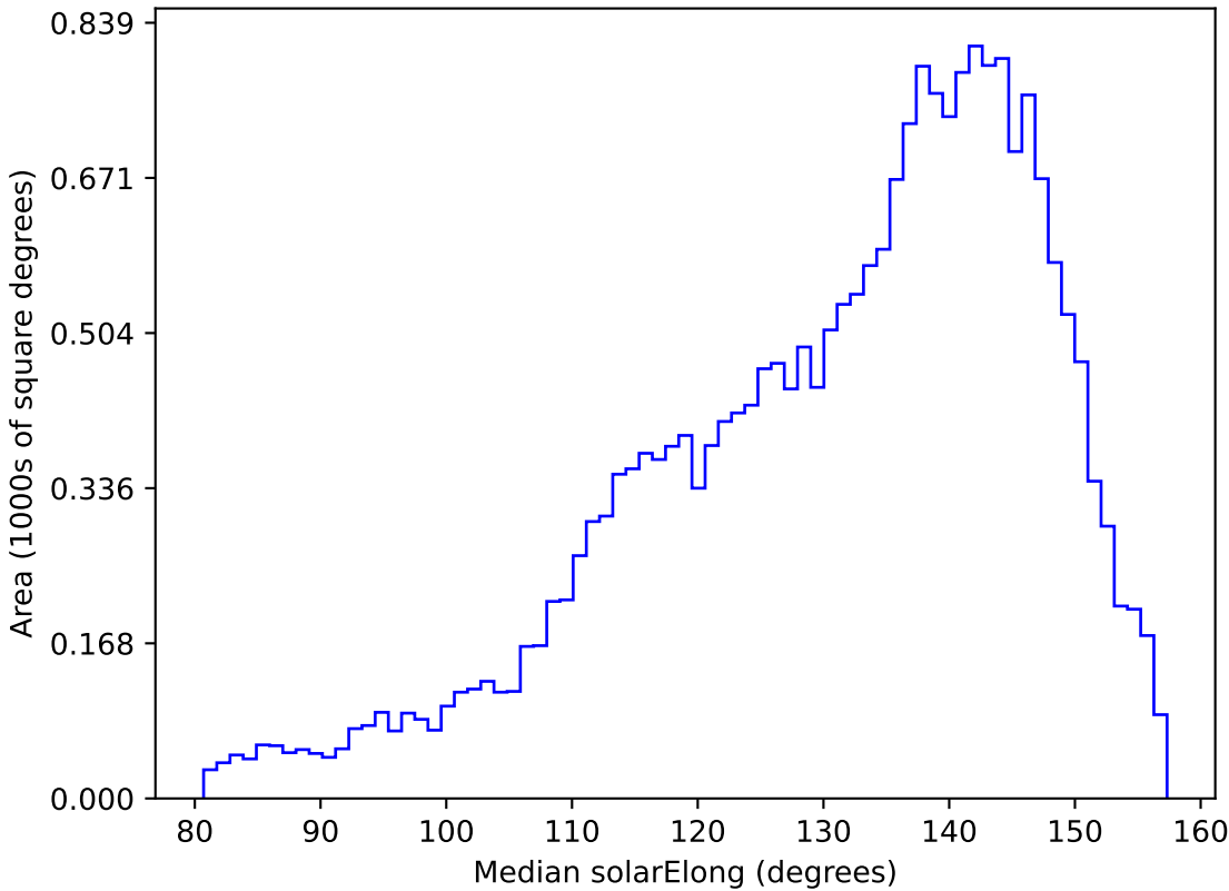
too_elab_r64_d2_gz_v3.4_10yrs All sky u band: Median solarElong
