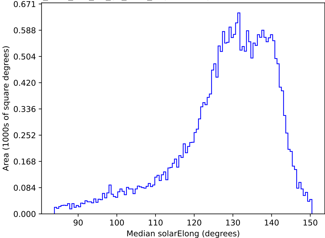
too_elab_r64_d2_gz_v3.4_10yrs All sky i band: Median solarElong
