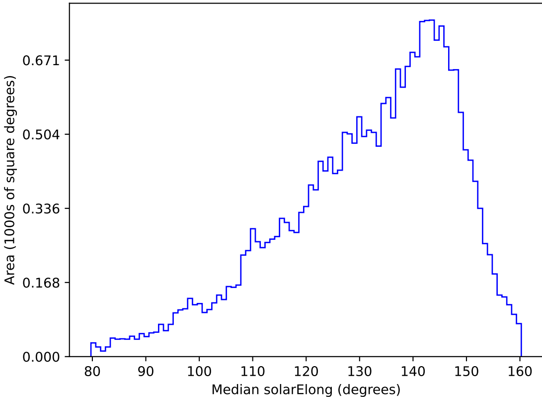
too_elab_r64_d2_gz_v3.4_10yrs All sky g band: Median solarElong
