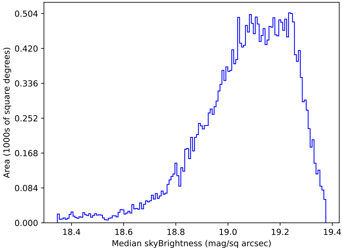
too_elab_r64_d2_gz_v3.4_10yrs Yr 1 z band: Median skyBrightness
