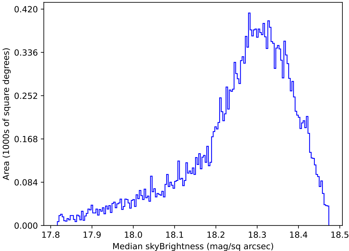
too_elab_r64_d2_gz_v3.4_10yrs Yr 1 y band: Median skyBrightness
