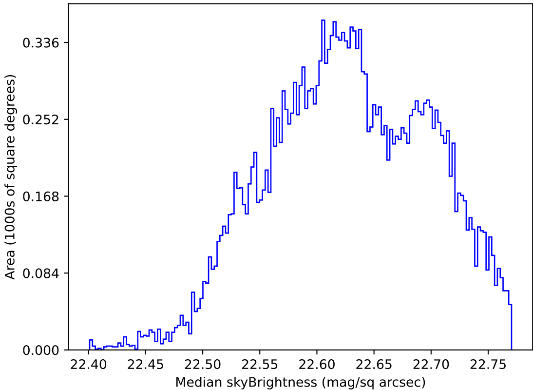
too_elab_r64_d2_gz_v3.4_10yrs Yr 1 u band: Median skyBrightness
