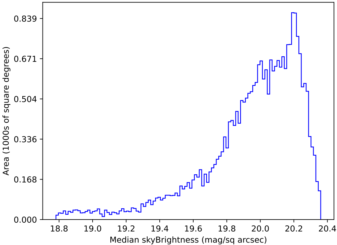
too_elab_r64_d2_gz_v3.4_10yrs Yr 1 i band: Median skyBrightness
