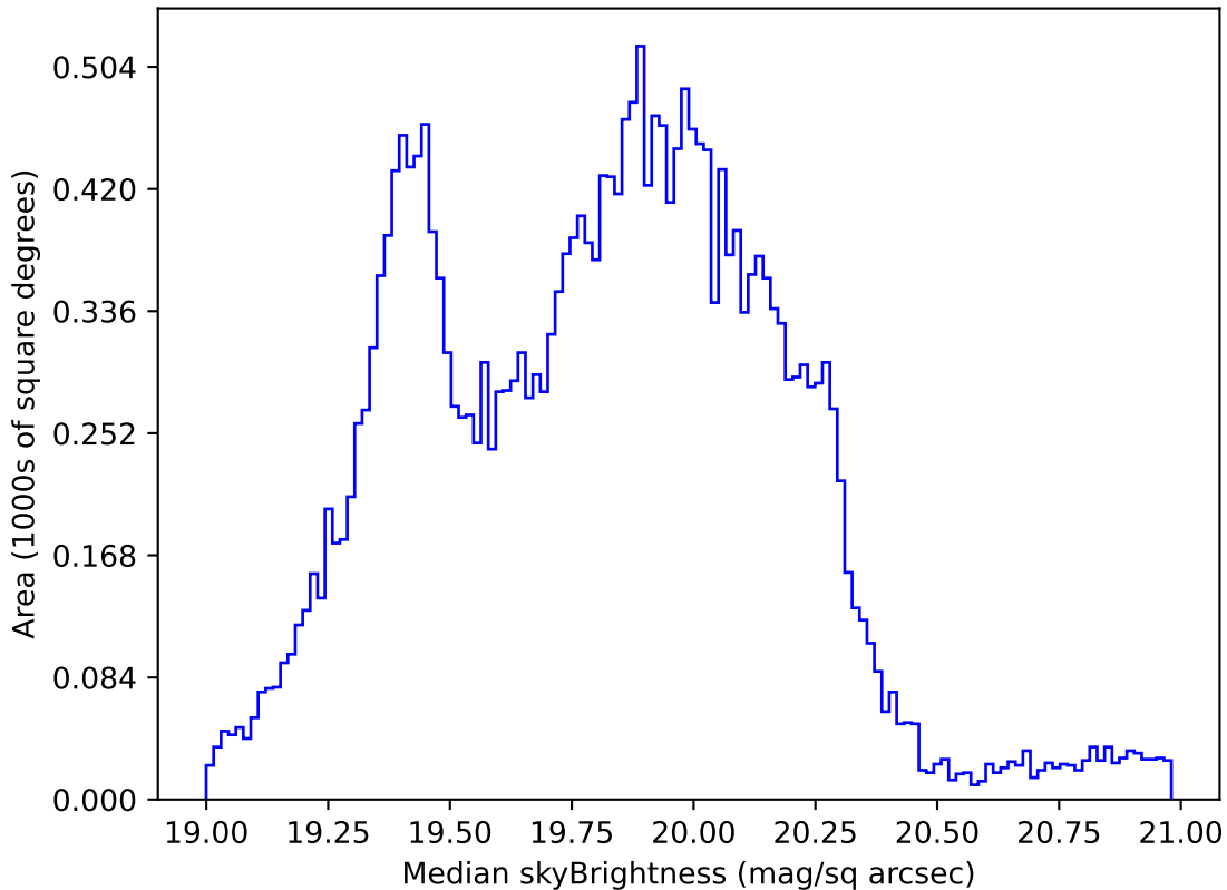
too_elab_r64_d2_gz_v3.4_10yrs Yr 1 all bands: Median skyBrightness
