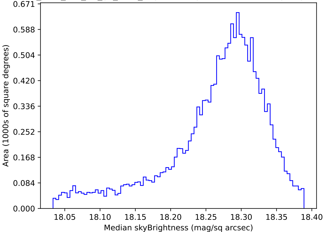
too_elab_r64_d2_gz_v3.4_10yrs WFD y band: Median skyBrightness
