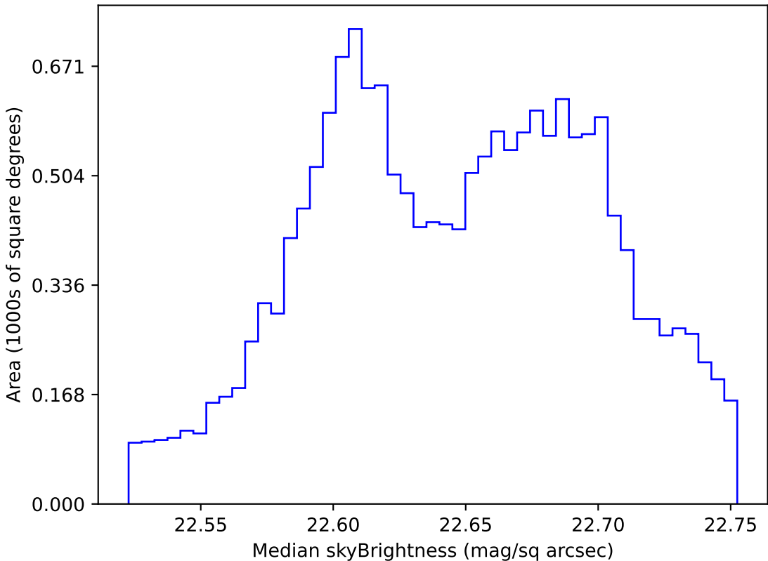
too_elab_r64_d2_gz_v3.4_10yrs WFD u band: Median skyBrightness
