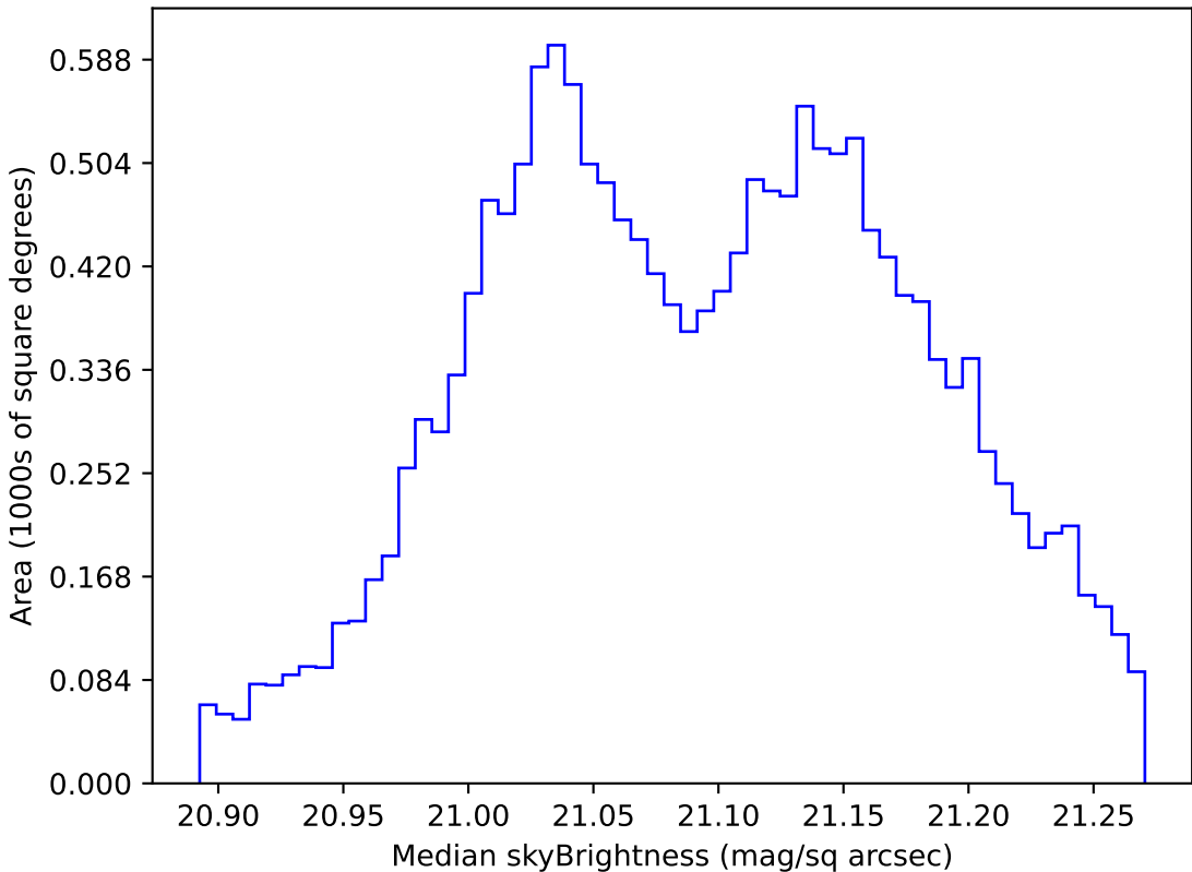
too_elab_r64_d2_gz_v3.4_10yrs WFD r band: Median skyBrightness
