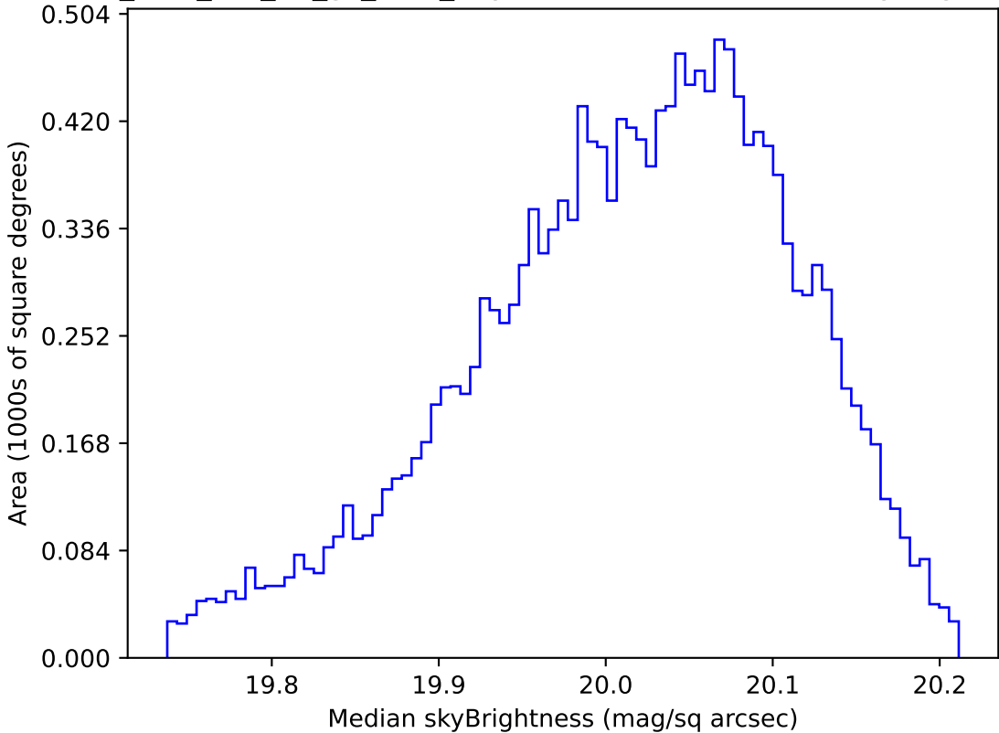
too_elab_r64_d2_gz_v3.4_10yrs WFD i band: Median skyBrightness
