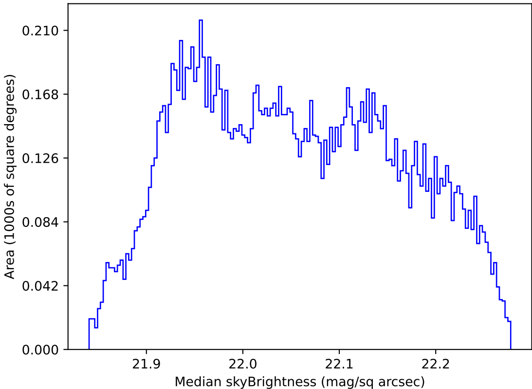
too_elab_r64_d2_gz_v3.4_10yrs WFD g band: Median skyBrightness
