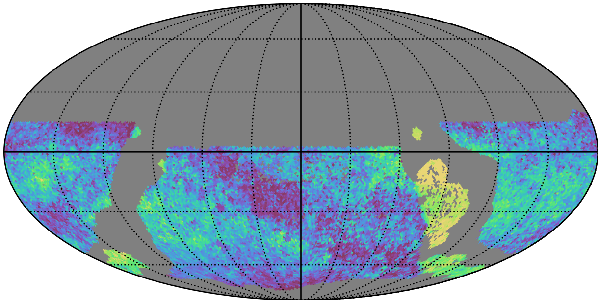
too_elab_r64_d2_gz_v3.4_10yrs WFD all bands: Median skyBrightness
