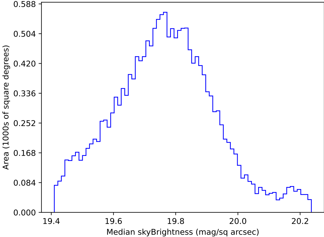
too_elab_r64_d2_gz_v3.4_10yrs WFD all bands: Median skyBrightness
