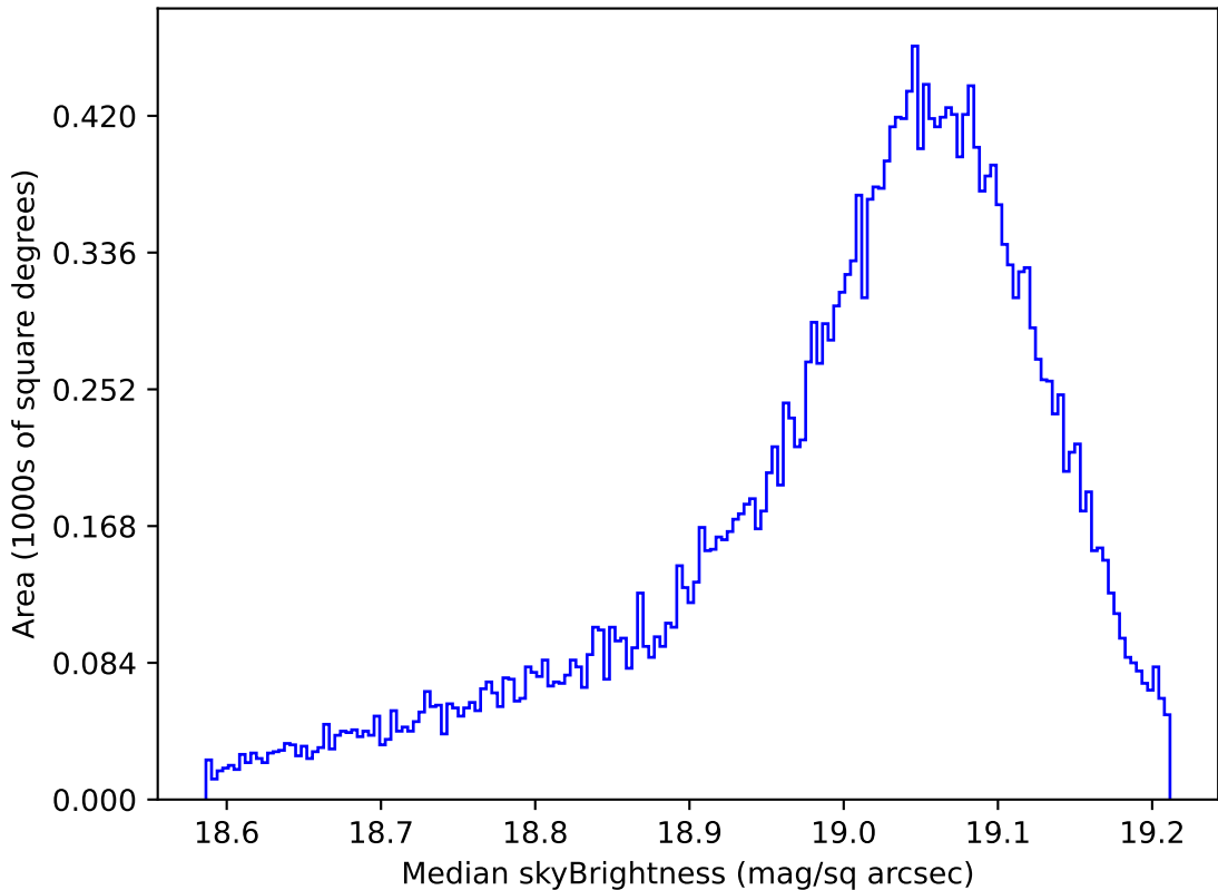
too_elab_r64_d2_gz_v3.4_10yrs All sky z band: Median skyBrightness
