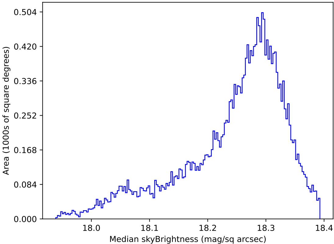
too_elab_r64_d2_gz_v3.4_10yrs All sky y band: Median skyBrightness
