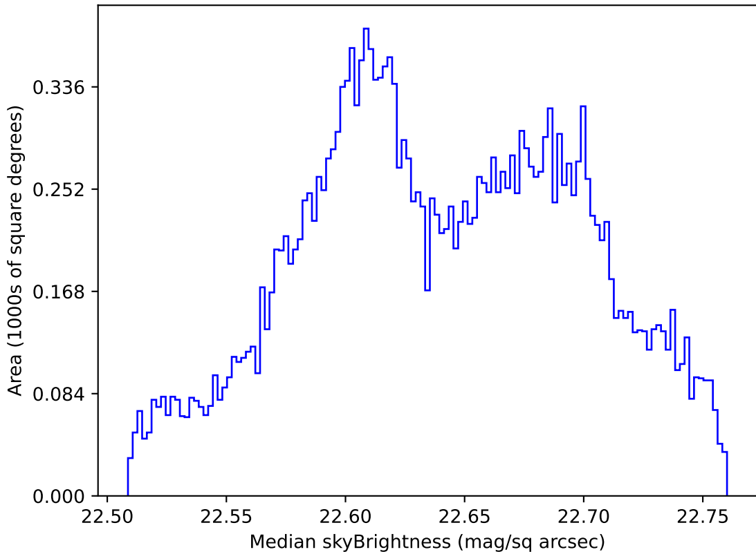
too_elab_r64_d2_gz_v3.4_10yrs All sky u band: Median skyBrightness
