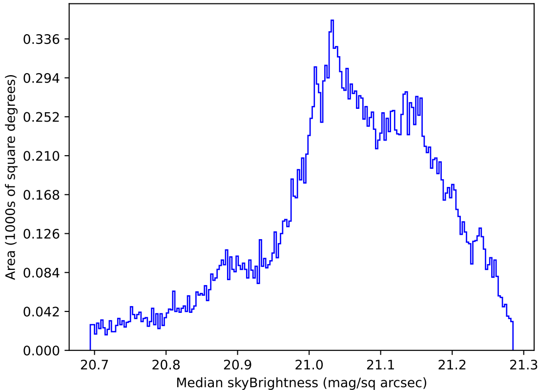
too_elab_r64_d2_gz_v3.4_10yrs All sky r band: Median skyBrightness
