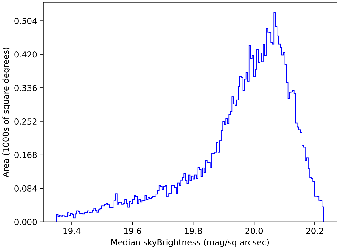
too_elab_r64_d2_gz_v3.4_10yrs All sky i band: Median skyBrightness
