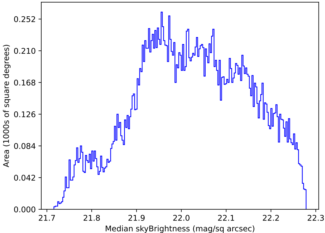
too_elab_r64_d2_gz_v3.4_10yrs All sky g band: Median skyBrightness
