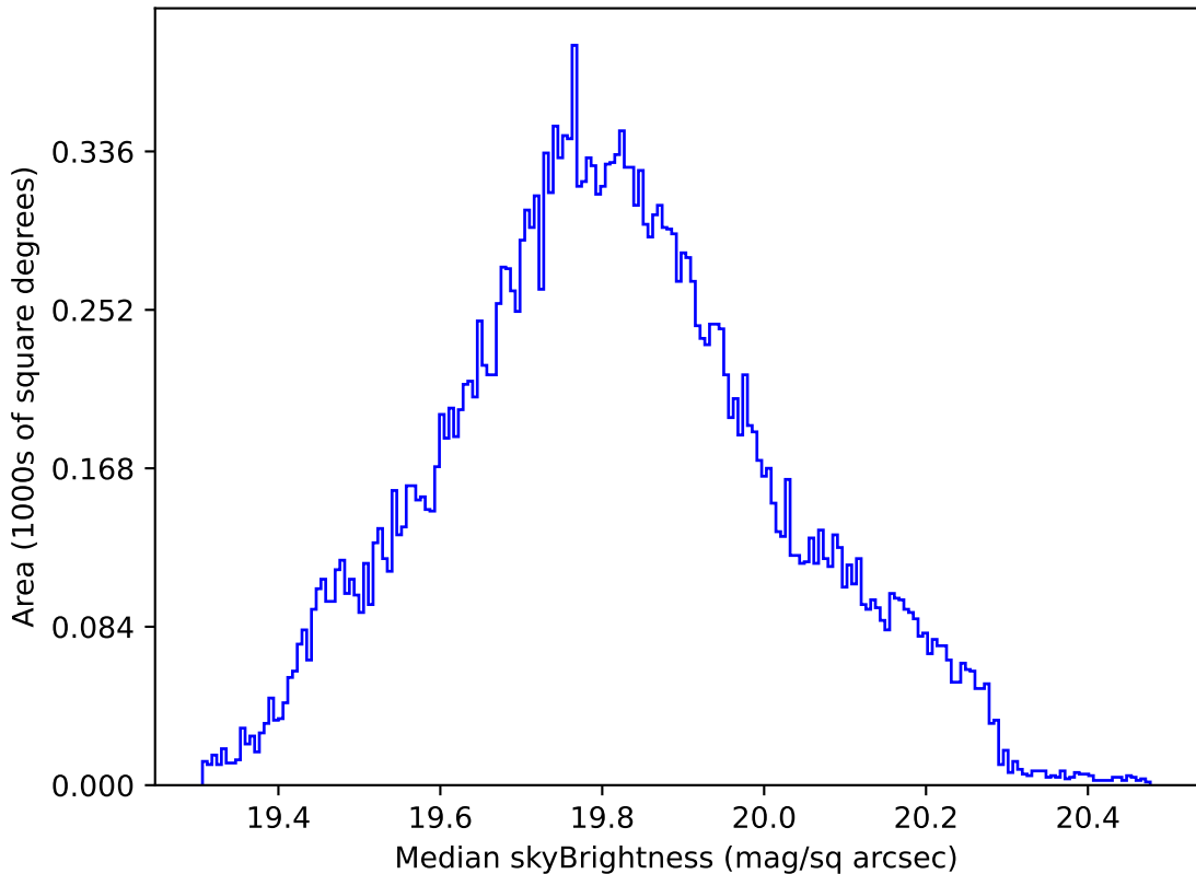
too_elab_r64_d2_gz_v3.4_10yrs All sky all bands: Median skyBrightness
