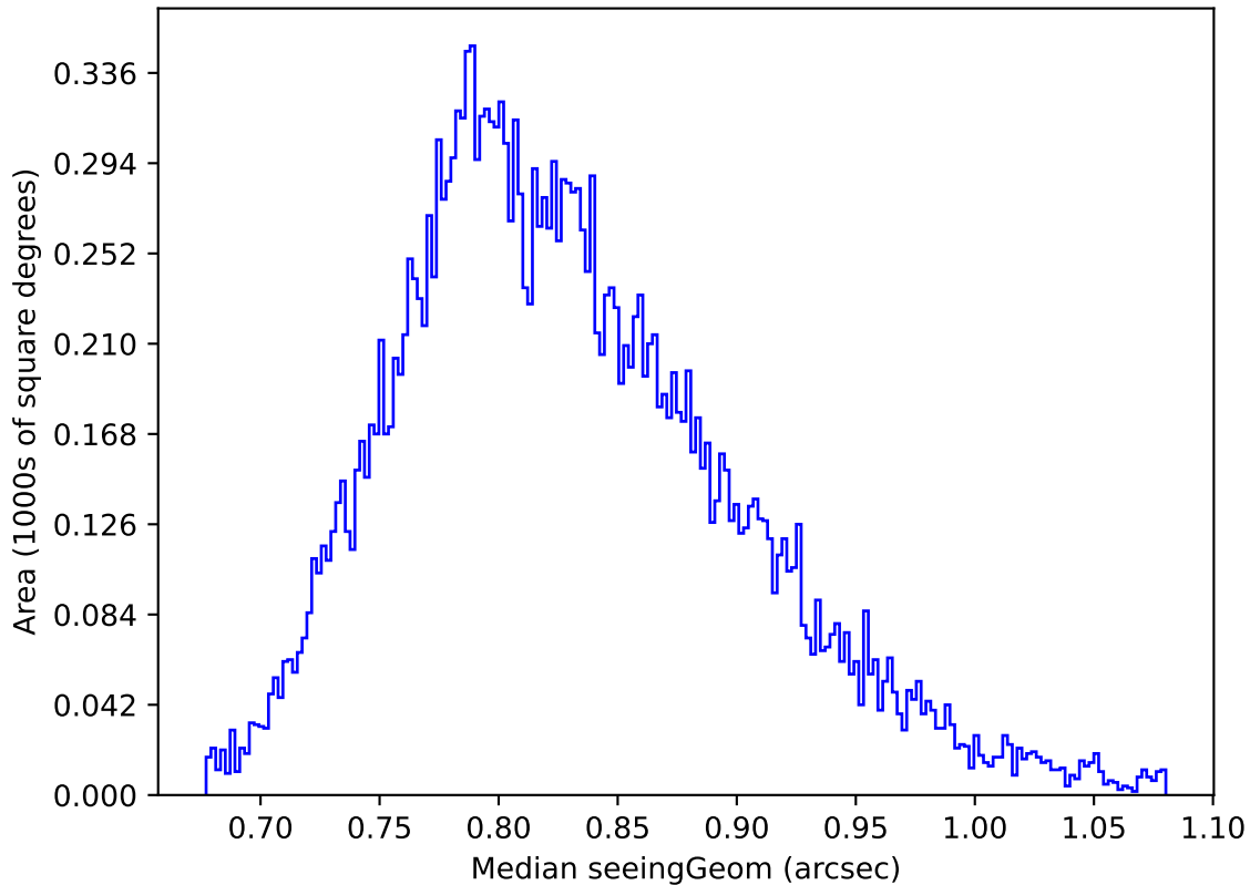
too_elab_r64_d2_gz_v3.4_10yrs Yr 1 y band: Median seeingGeom
