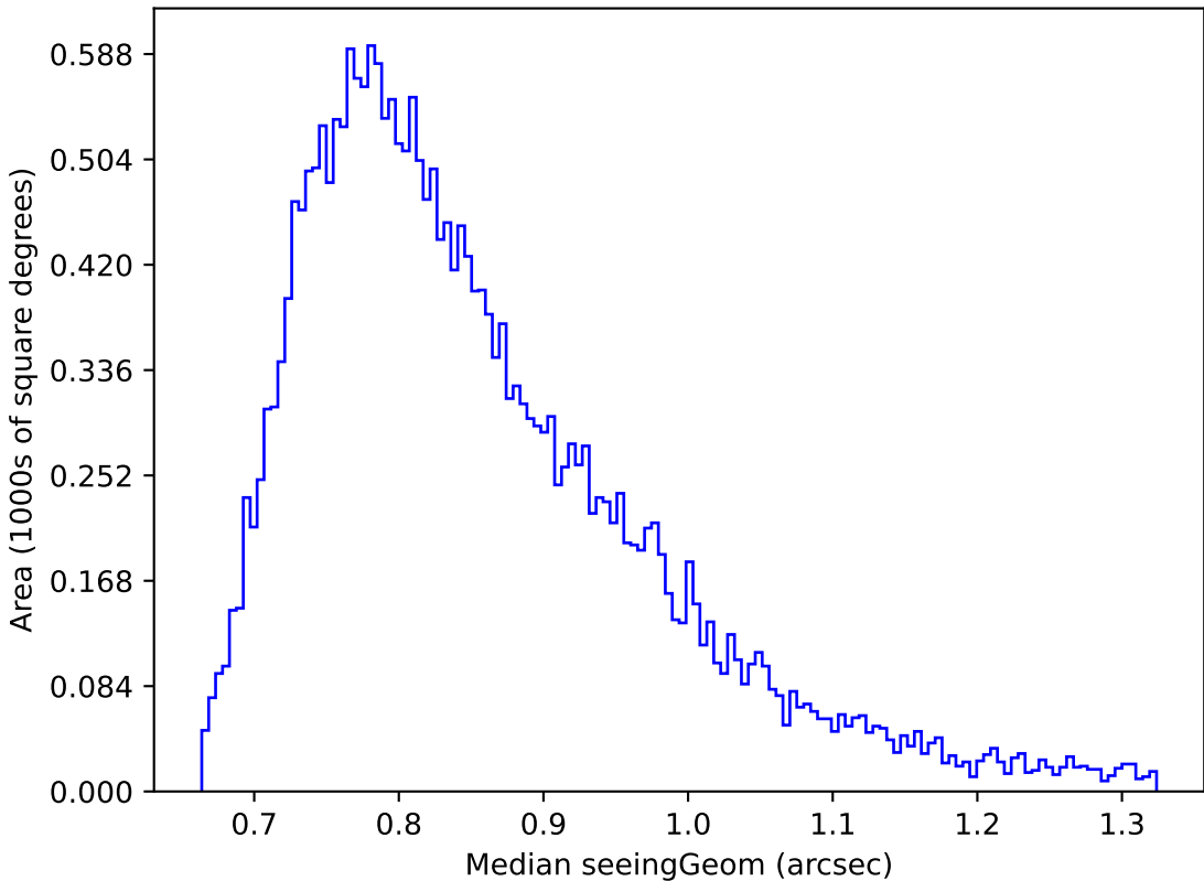
too_elab_r64_d2_gz_v3.4_10yrs Yr 1 r band: Median seeingGeom
