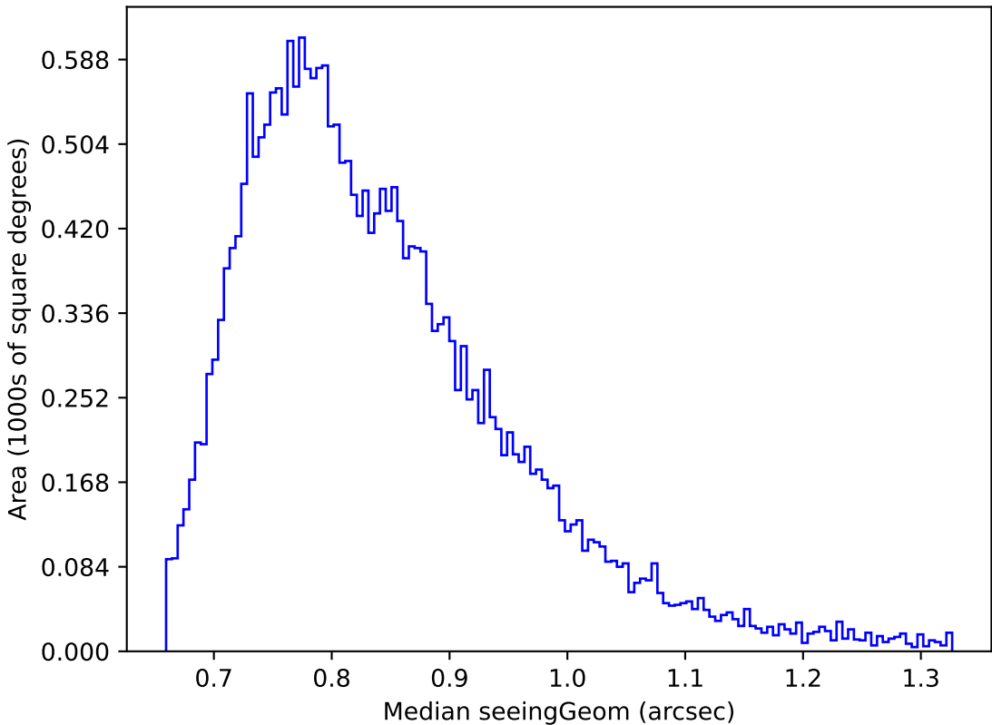
too_elab_r64_d2_gz_v3.4_10yrs Yr 1 i band: Median seeingGeom
