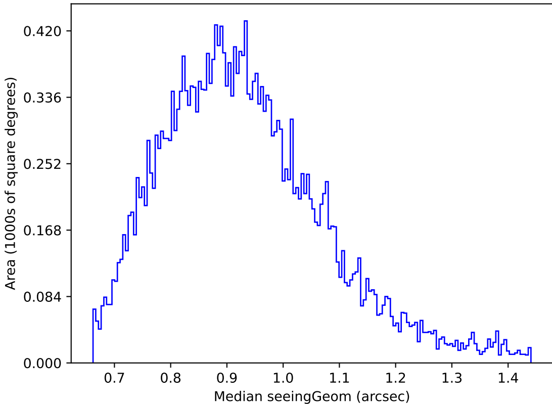
too_elab_r64_d2_gz_v3.4_10yrs Yr 1 g band: Median seeingGeom
