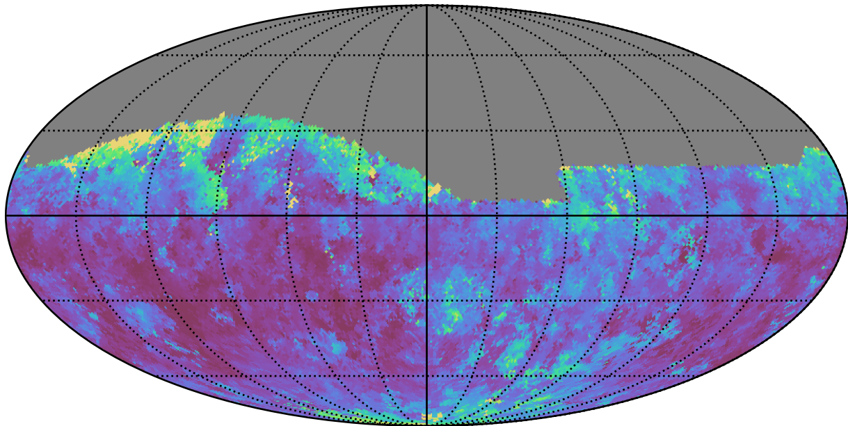
too_elab_r64_d2_gz_v3.4_10yrs Yr 1 z band: Median seeingEff
