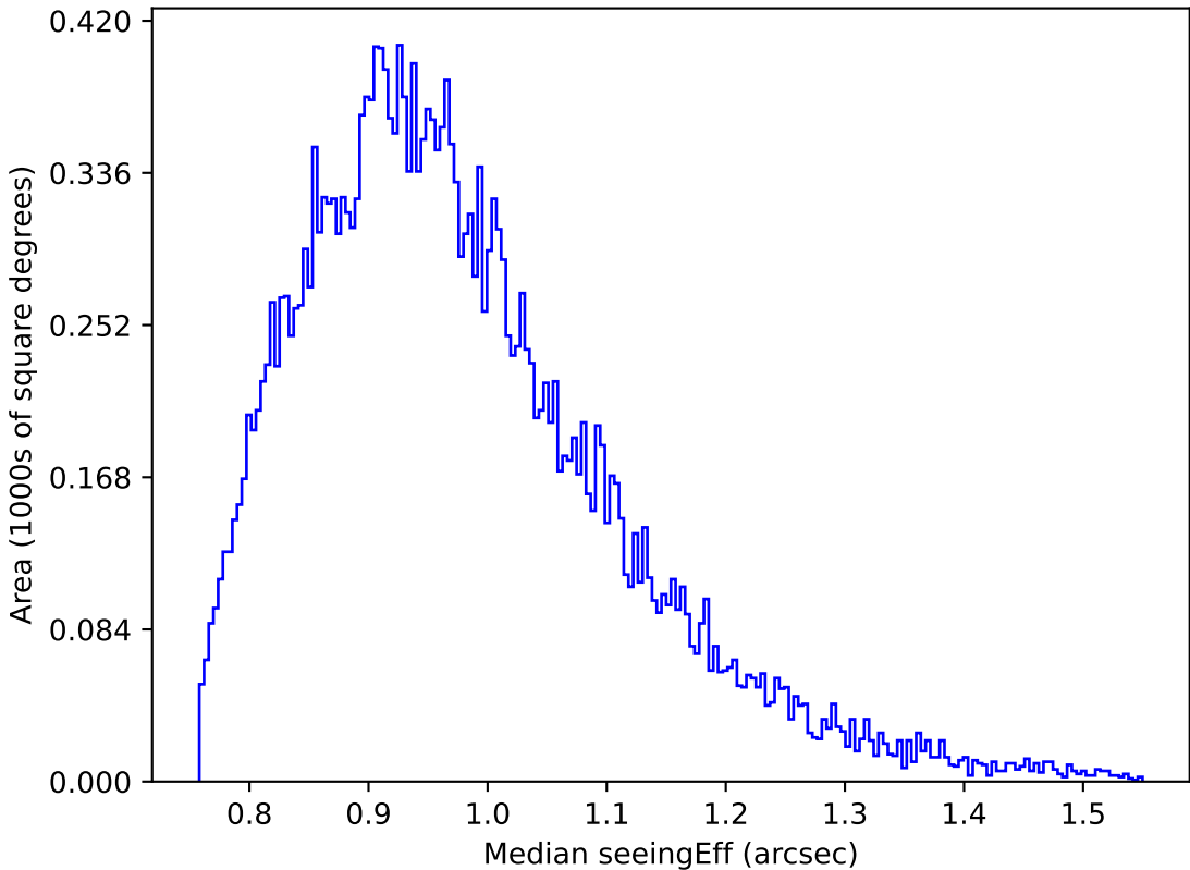
too_elab_r64_d2_gz_v3.4_10yrs Yr 1 z band: Median seeingEff
