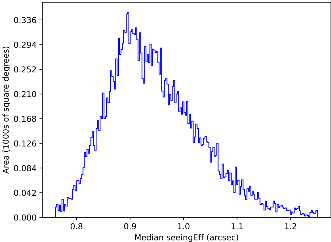
too_elab_r64_d2_gz_v3.4_10yrs Yr 1 y band: Median seeingEff
