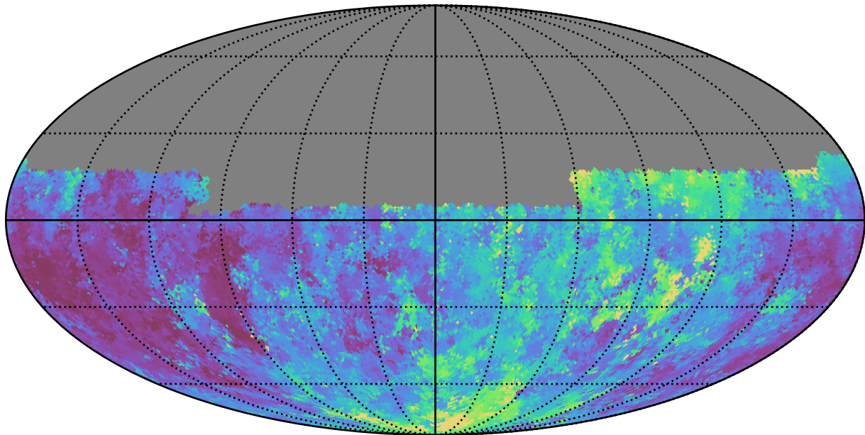
too_elab_r64_d2_gz_v3.4_10yrs Yr 1 u band: Median seeingEff
