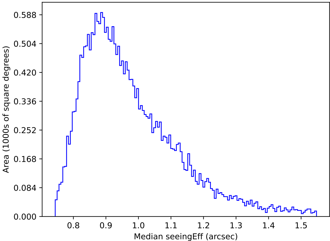
too_elab_r64_d2_gz_v3.4_10yrs Yr 1 r band: Median seeingEff
