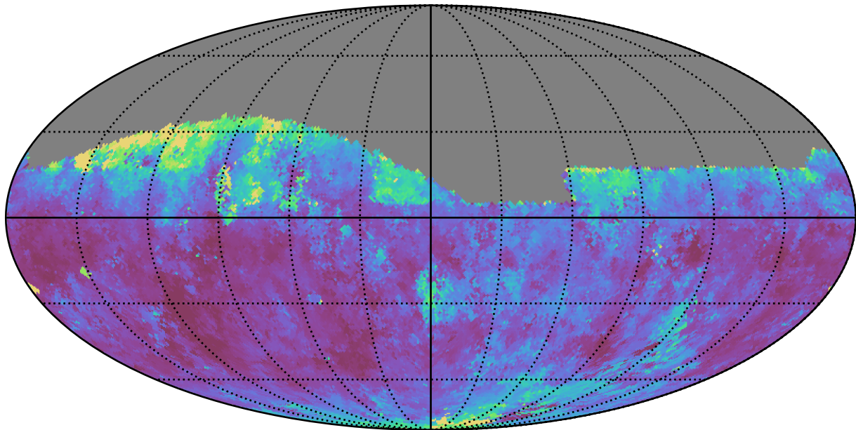
too_elab_r64_d2_gz_v3.4_10yrs Yr 1 i band: Median seeingEff
