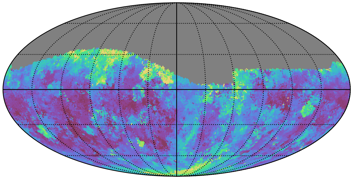
too_elab_r64_d2_gz_v3.4_10yrs Yr 1 g band: Median seeingEff
