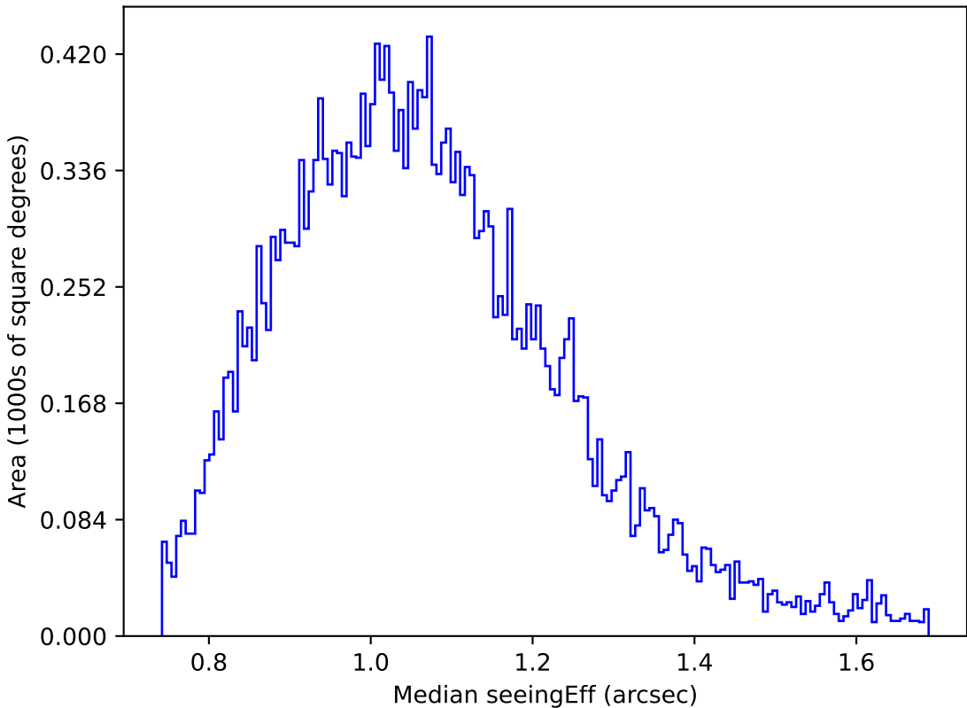
too_elab_r64_d2_gz_v3.4_10yrs Yr 1 g band: Median seeingEff
