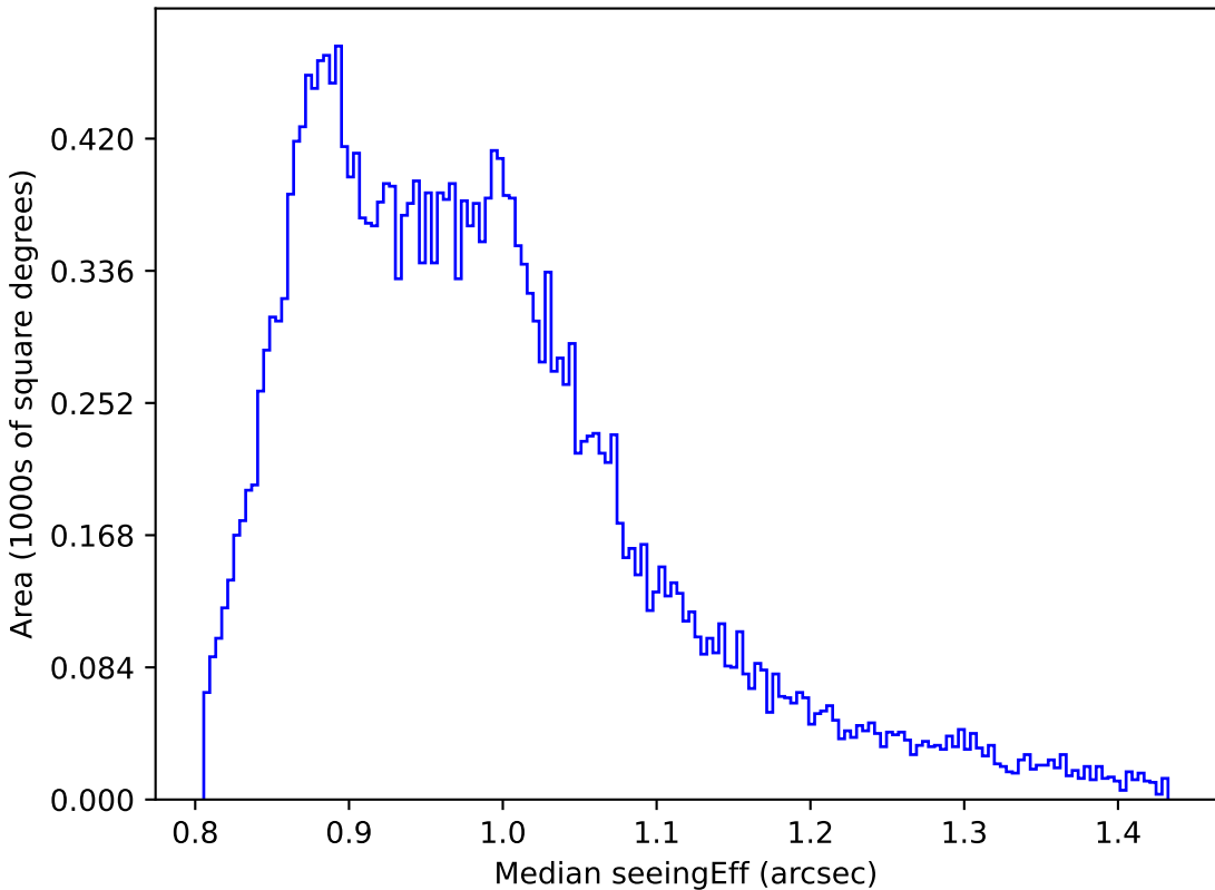
too_elab_r64_d2_gz_v3.4_10yrs Yr 1 all bands: Median seeingEff
